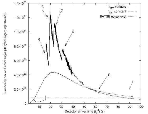
FIG. 5.—Source luminosity connected to the mask in Fig. 3 given as a function of the detector arrival time (solid “spiky” line), with the corresponding curve for the case of constant n_{\text{ISM}} = 1 \text{ particle cm}^{-3} (smooth dashed line) and the BATSE noise level (horizontal dotted line). The “noise” observed in the theoretical curves is due to the discretization process adopted, described in Ruffini et al. (2002b), for the description of the angular spreading of the scattered radiation. For each fixed value of the laboratory time, we have summed 500 different contributions from different angles. The integration of the equation of motion of this system is performed in 22,314,500 contributions to be considered. An increase in the number of steps and in the precision of the numerical computation would lead to a smoother curve.
