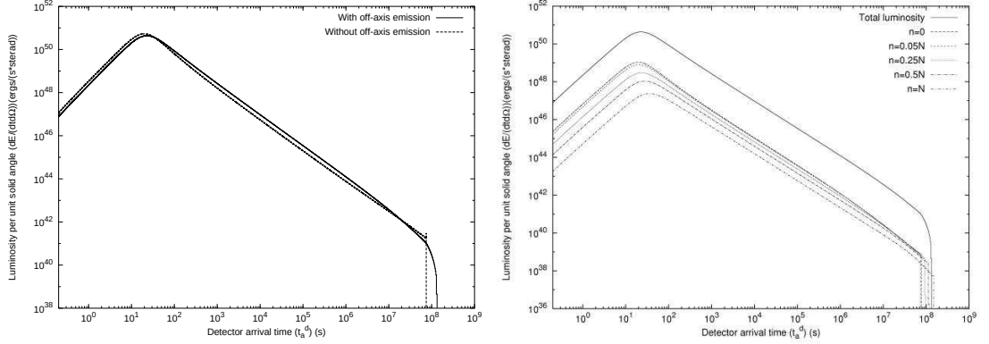
Figure 14: Left) The predicted afterglow curve for GRB 991216 assuming a constant ISM density equal to 1 \text{ particle/cm}^3 and taking into account all the effects due to off-axis emission (solid line). For comparison we plot also the corresponding curve obtained in the simple radial approximation (dashed line). We see that this last curve falls sharply to zero when the ABM pulse reaches \gamma = 1 , while the first one has a much smoother behavior due to the time delay in the arrival of the photons emitted at large \vartheta . Recall that when \gamma tends to 1, the maximum allowed values of \vartheta tend to 90^\circ . Right) This figure shows how the radiation emitted from different angles contributes to the afterglow luminosity. The solid line on the top of the picture is the total luminosity as in the previous plots. The other dashed and dotted curves represent the radiation components corresponding to selected values of n in Eq.(181). From the upper to the lower one they corresponds respectively to n = 0 , n = 0.05N , n = 0.25N , n = 0.5N , n = N , where in this plot N = 200 . We can easily see that the radiation emitted at large angles ( n = N ) is time shifted with respect to that emitted near the line of sight ( n = 0 ).
