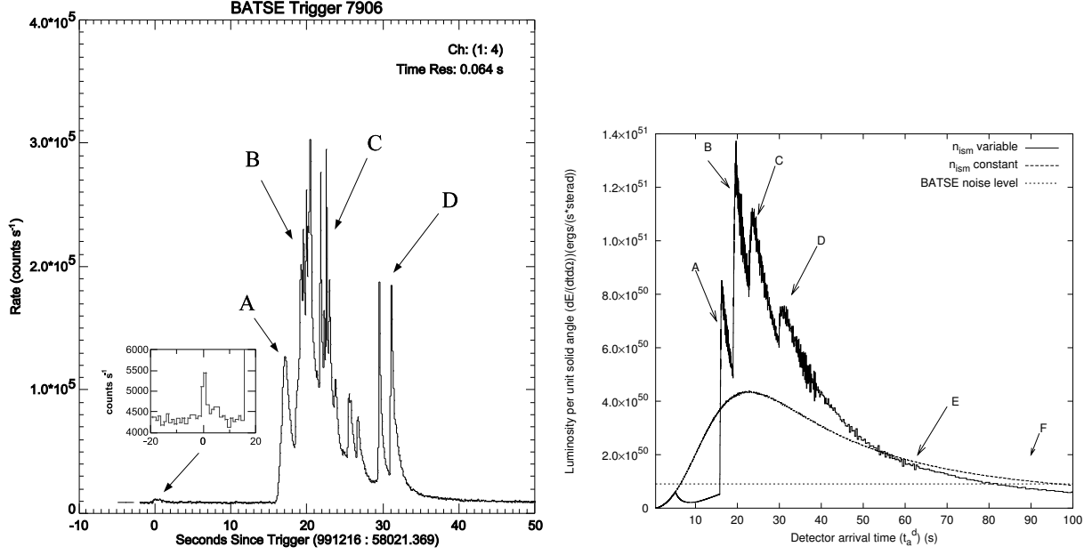
Figure 4.12: Left) The BATSE data on the E-APE of GRB 991216 (source: [6]) together with an enlargement of the P-GRB data (source: [7]). For convenience each E-APE peak has been labeled by a different uppercase Latin letter. Right) The source luminosity corresponding to the mask in fig. 4.10 is given as a function of the detector arrival time (solid “spiky” line) with the corresponding curve for the case of constant \langle n_{\text{ism}} \rangle = 3 \text{ particle/cm}^3 (dashed smooth line) and the BATSE noise level (dotted horizontal line).
