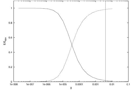
FIG. 4.—Relative intensities of the afterglow (dashed line) and the P-GRB (solid line), as predicted by the EMBH model corresponding to the values of the parameters determined in Fig. 3, as a function of B . Details are given in (Bianco et al. 2001a). The vertical line corresponds to the value B = 4 \times 10^{-3} .
