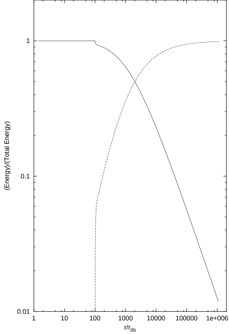
Fig. 26. The energy of the non-baryonic components of the PEMB pulse (the solid line) and the kinetic energy of the baryonic matter (the dashed line) in the unit of the total energy are plotted as functions of the radius in the unit of the dyadosphere radius r_{\text{ds}} .
