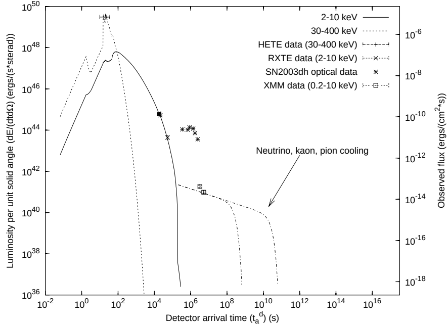
FIGURE 1. The dotted line represents our theoretically predicted GRB030329 light curve in \gamma -rays (30-400 keV) with the horizontal bar corresponding to the mean peak flux from HETE-2 (gc1 [1]). The solid line represents the corresponding one in X-rays (2-10 keV) with the experimental data obtained by R-XTE (gc2 [2]). The remaining points refer respectively to the optical VLT data (Hjorth et al. [4]) of SN2003bh and to the X-ray XMM data (Tiengo et al. [3]) of URCA-2. The dash-dotted lines corresponds to cooling theoretical curves of young neutron stars by generalized URCA processes. It is interesting to compare and contrast these results with the ones for GRB980425/SN1998bw (see Fig. 3 in Ruffini et al. [6])
